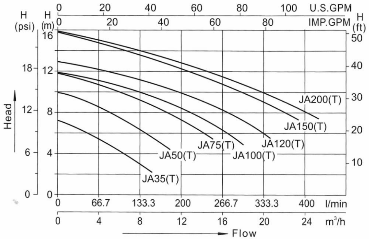
Performance curves
